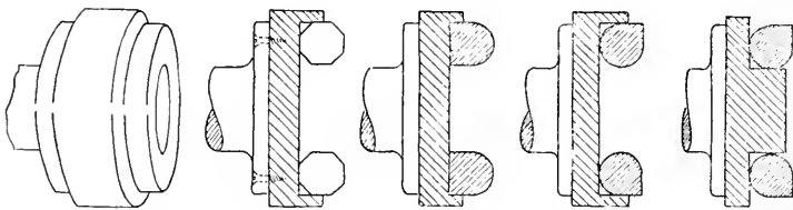
FIG. 325. TURNING A RING—FIRST METHOD.
